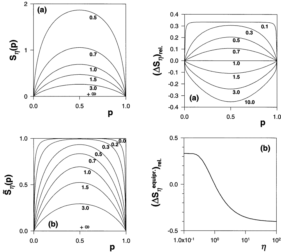
Figure 1. (a) Entropy S_\eta for a two-state system ( w = 2 ) as a function of p for different values of \eta indicated on the figure. (b) \tilde{S}_\eta \equiv S_\eta / \Gamma(\frac{\eta+1}{\eta}) versus p . Note that, as \eta decreases, S_\eta flattens around p = \frac{1}{2} .
